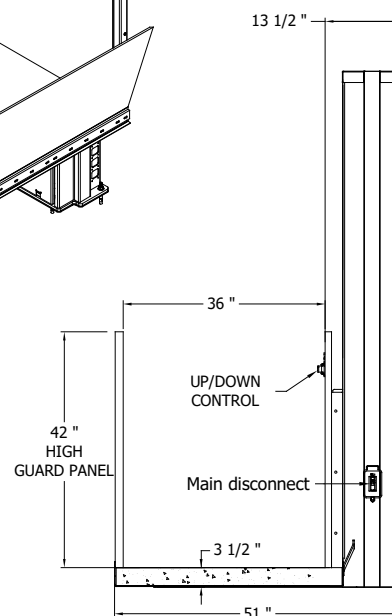
DETAIL B SIDE VIEW
