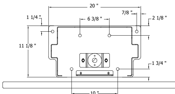
ANCHORAGE
