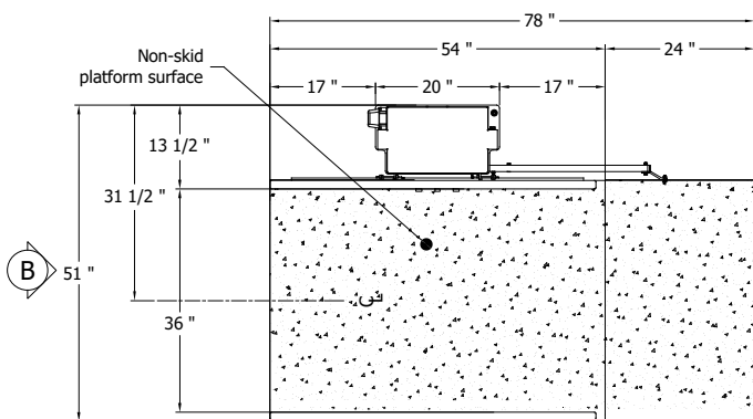
NANO 36X54 PLAN VIEW
