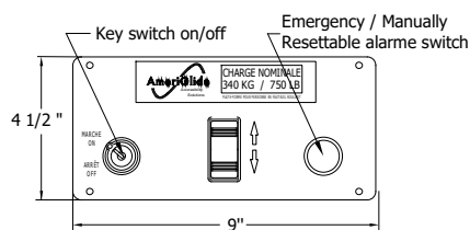
CONTROL PANEL
